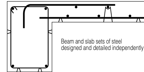
CORRECT DETAIL TO PREVENT THE FOLLOWING
