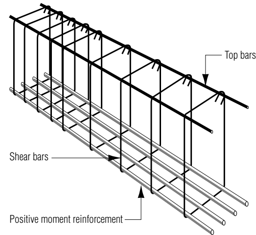
BASIC CAGE ARRANGEMENT
