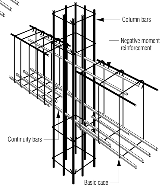
AFTER ASSEMBLY AT INTERSECTING COLUMN
